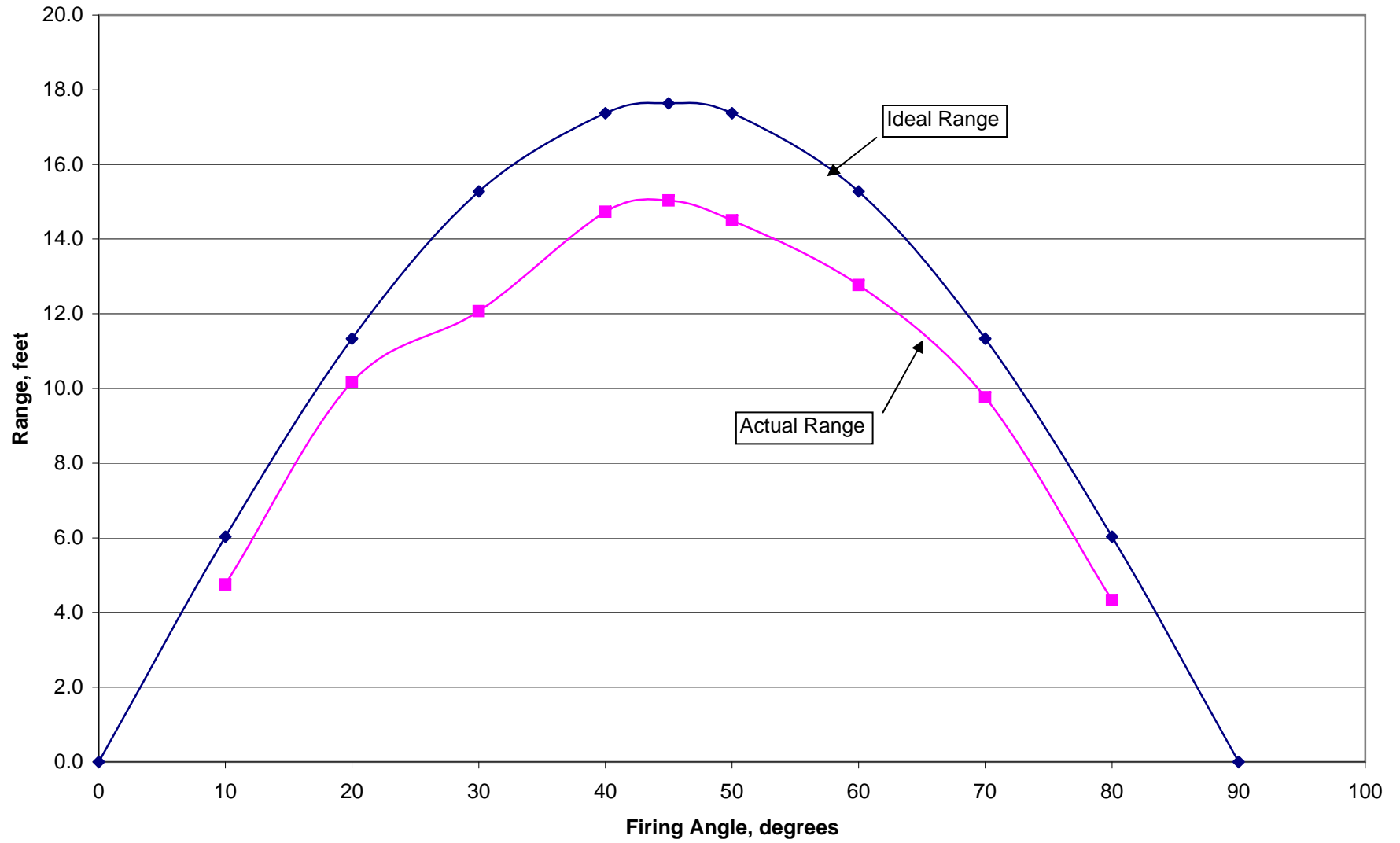
Ideal and Actual Range vs Firing Angle
