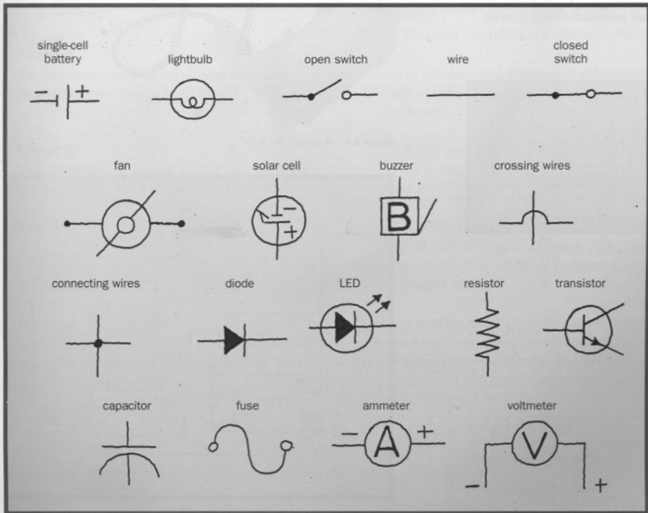
Figure 5.3 Electrical symbols chart
